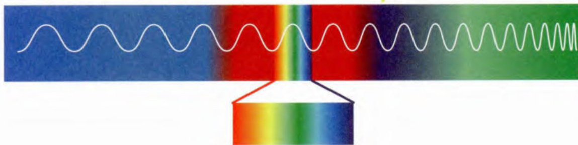
㉖ electromagnetic spectrum 电磁波谱
